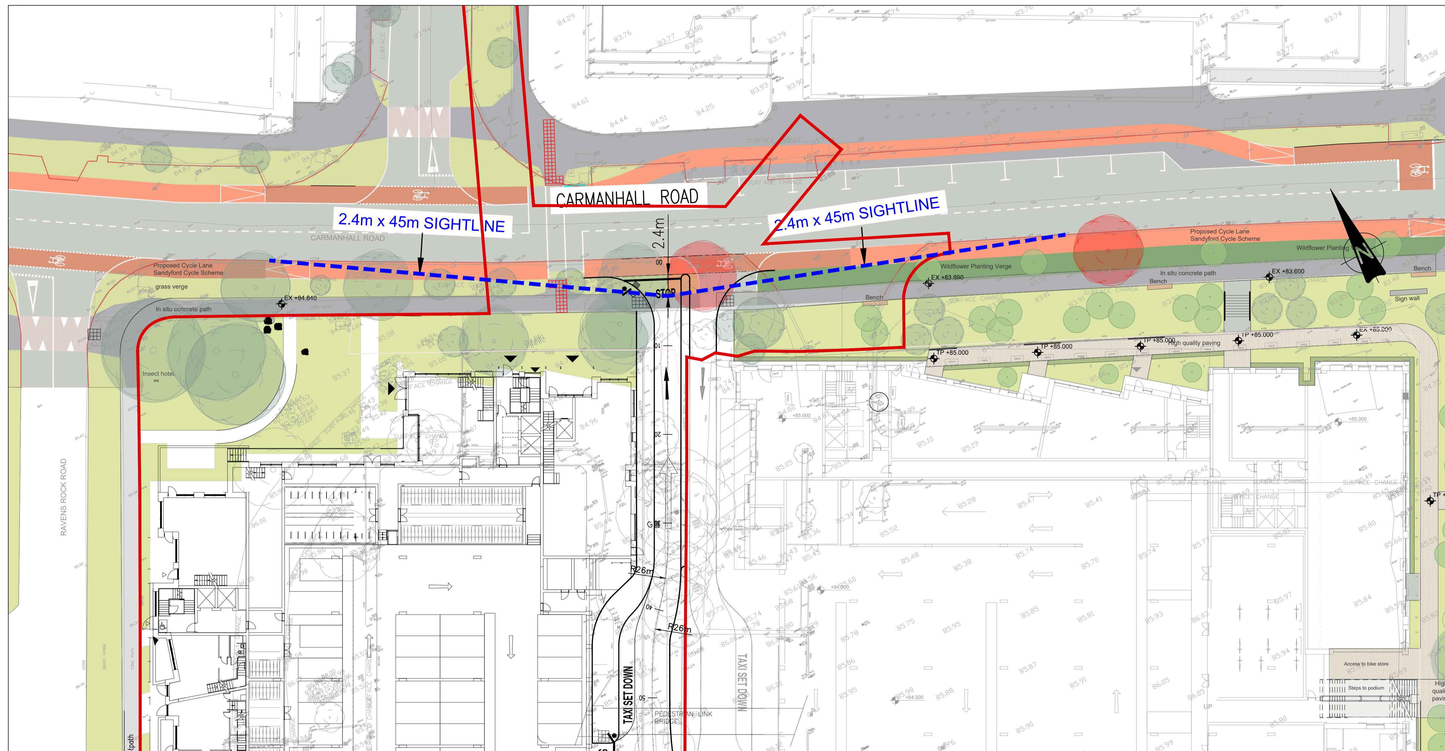
PLAN VIEW PROPOSED SIGHTLINES – CARMANHALL ROAD
